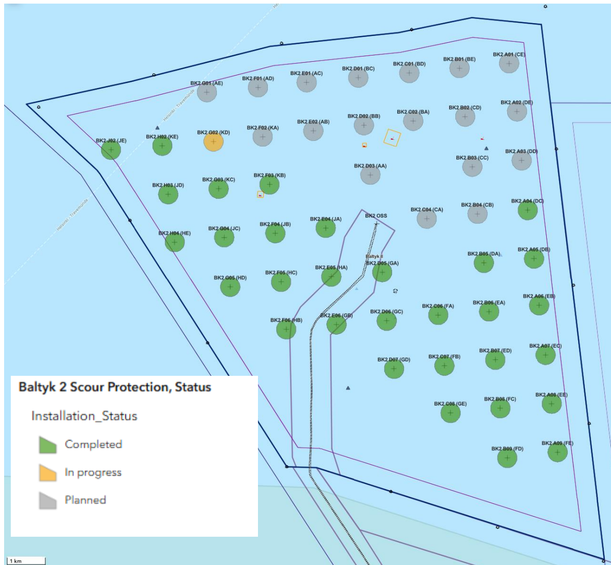
Figure 4 – Bałtyk 2 OWF Scour Protection Installation Overview (06.2.2026)
