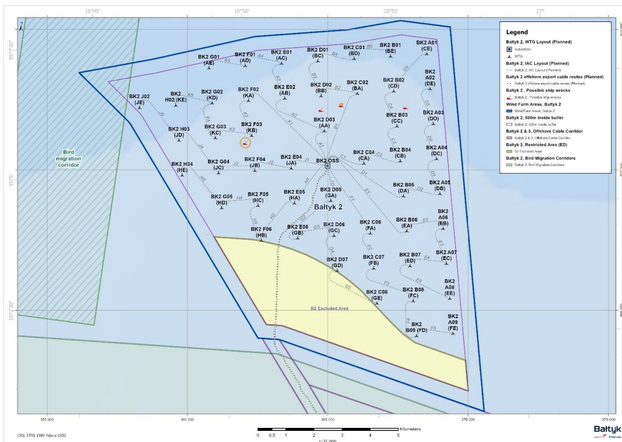
Figure 2 – Layout of the planned Bałtyk 2 OWF
