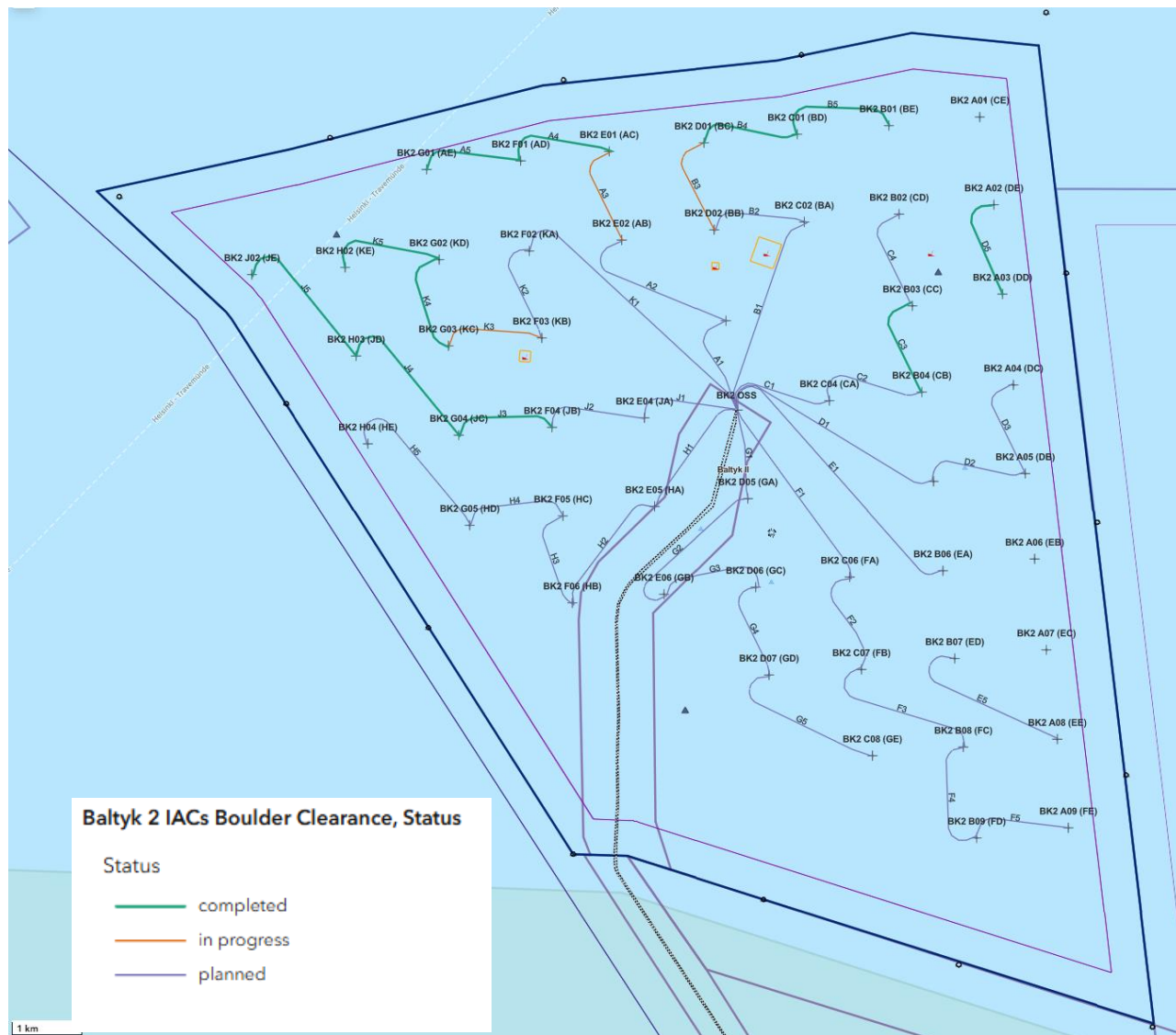
Figure 5 – Bałtyk 2 Inter Array Cables Boulder Clearance Status (06.2.2026)
