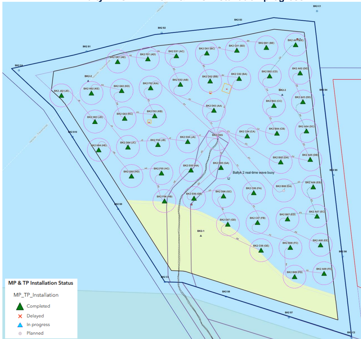
Figure 5 – Bałtyk 2 OWF Installation Overview
