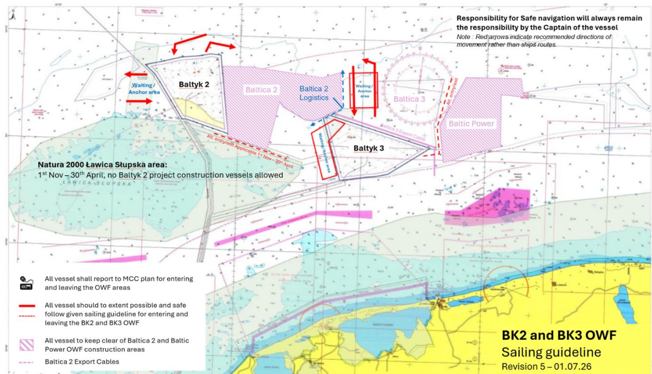
Figure 2 – Layout of the Bałyk 2&3 entry/exit corridors
