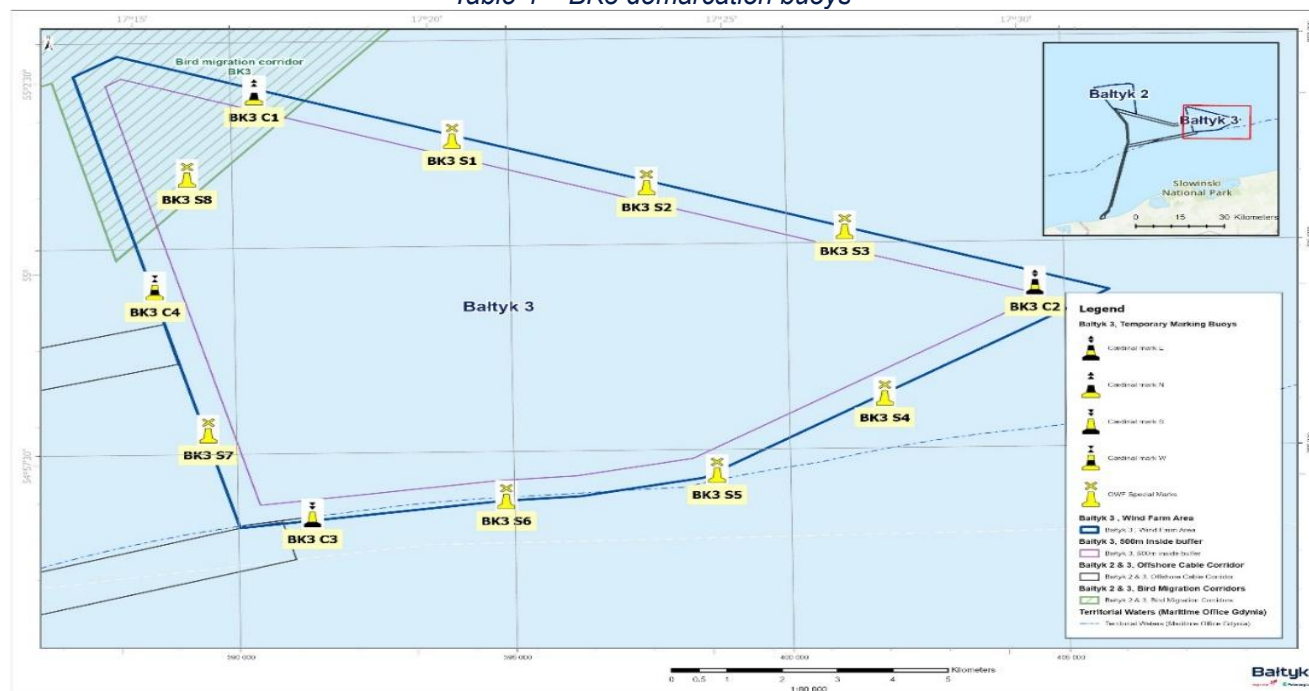
Figure 4 – Layout of demarcation buoys in Bałyk 3 OWF
