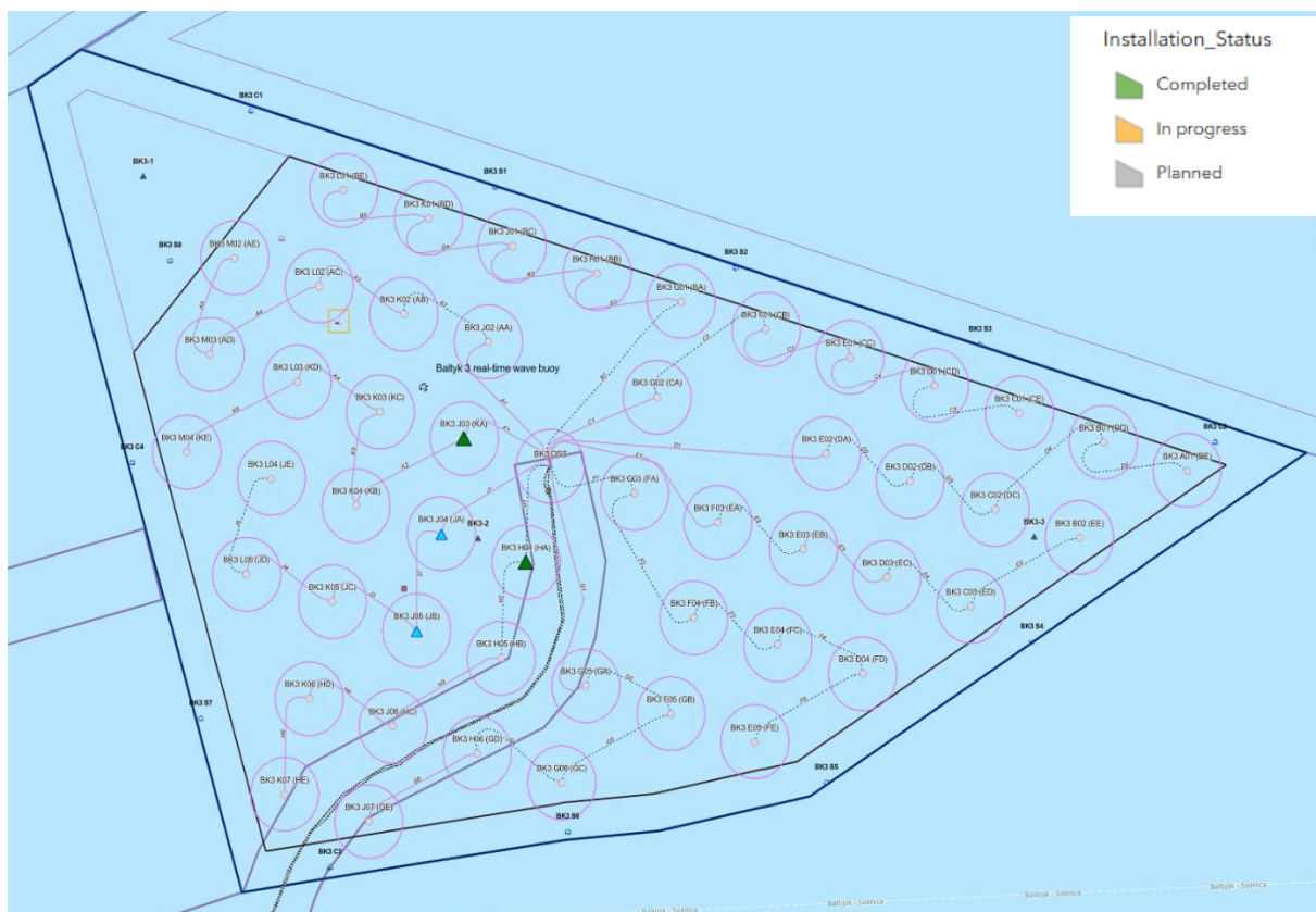
Figure 7 – Bałtyk 3 OWF Installation Overview
