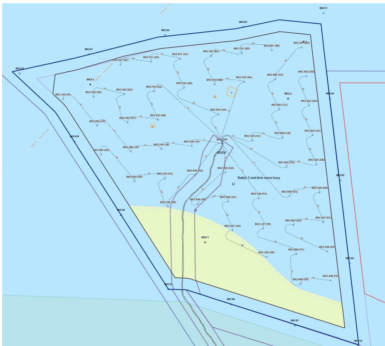
Figure 6 – Bałyk 2 Inter Array Cables Installation Status
