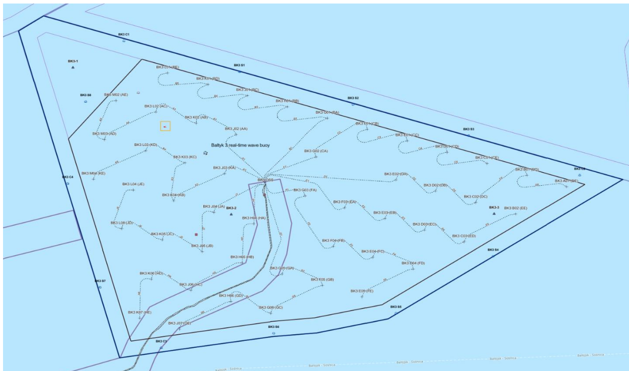
Figure 8 – Bałtyk 3 Inter Array Cables Installation Progress Status
