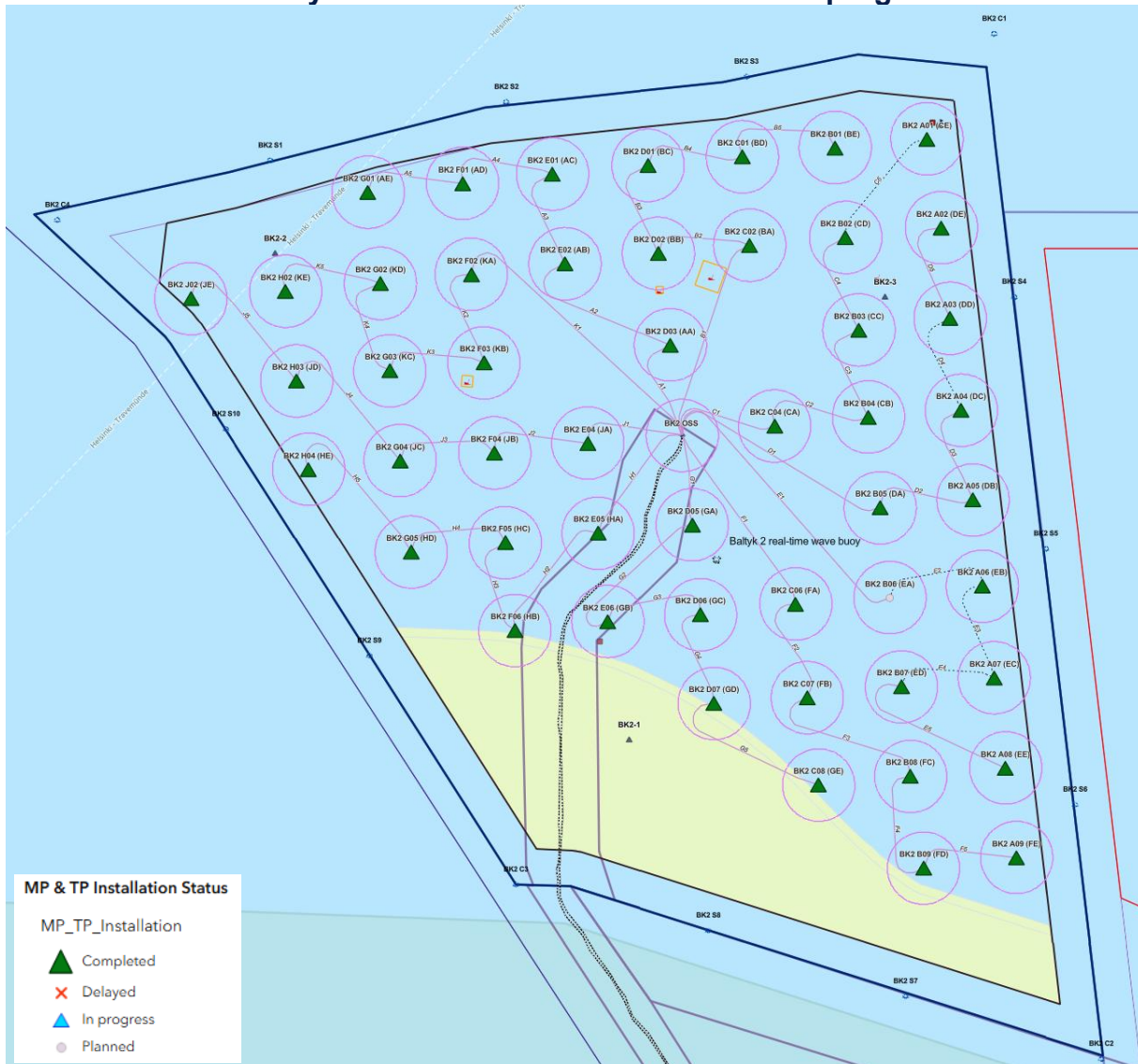
Figure 5 – Bałyk 2 OWF Installation Overview
