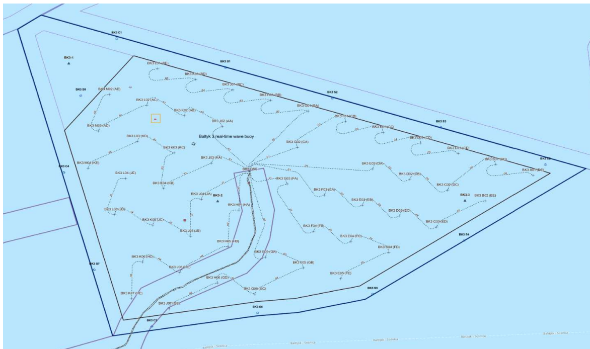
Figure 8 – Bałtyk 3 Inter Array Cables Installation Progress Status
