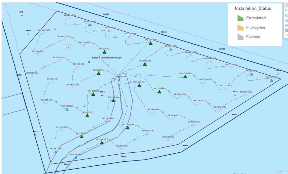
Figure 7 – Bałyk 3 OWF Installation Overview
