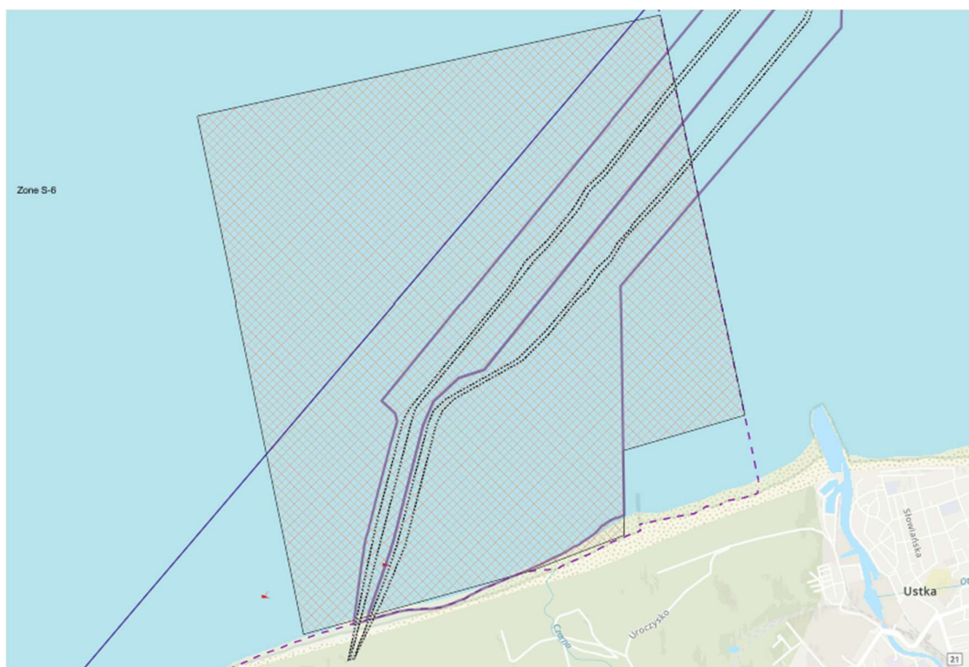
Figure 9 – Bałtyk 2&3 export cables construction area safety zone
