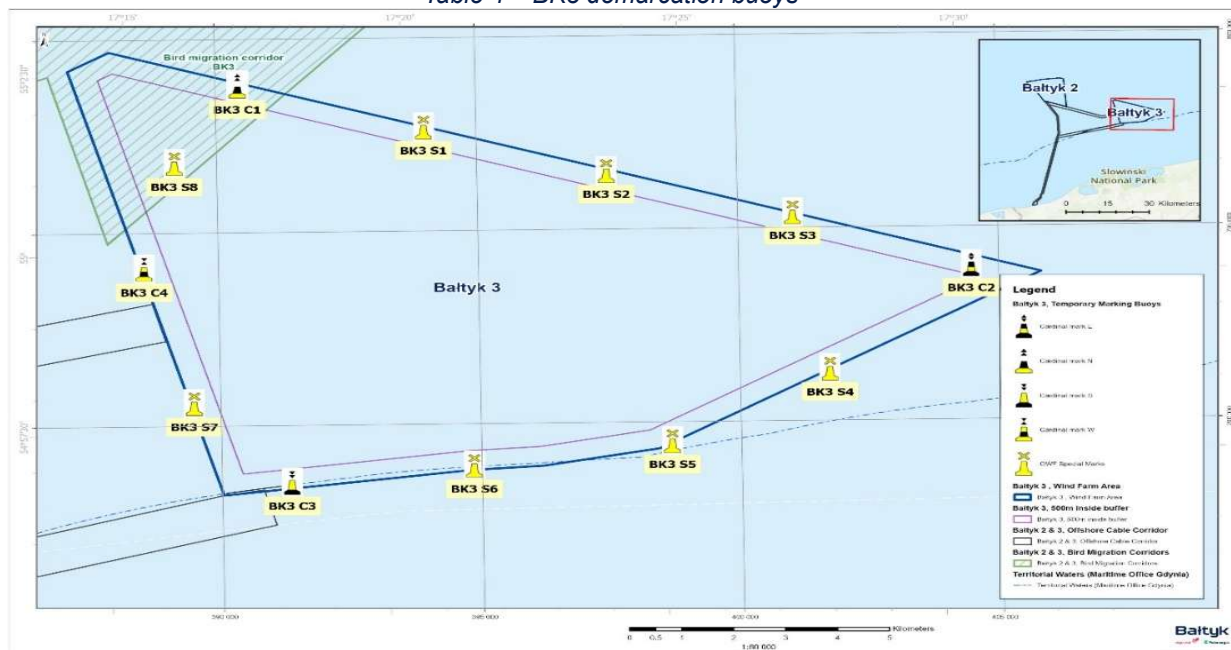
Figure 4 – Layout of demarcation buoys in Bałtyk 3 OWF
