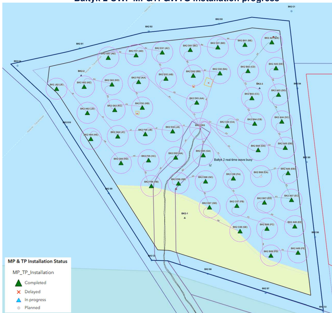
Figure 5 – Bałtyk 2 OWF Installation Overview
