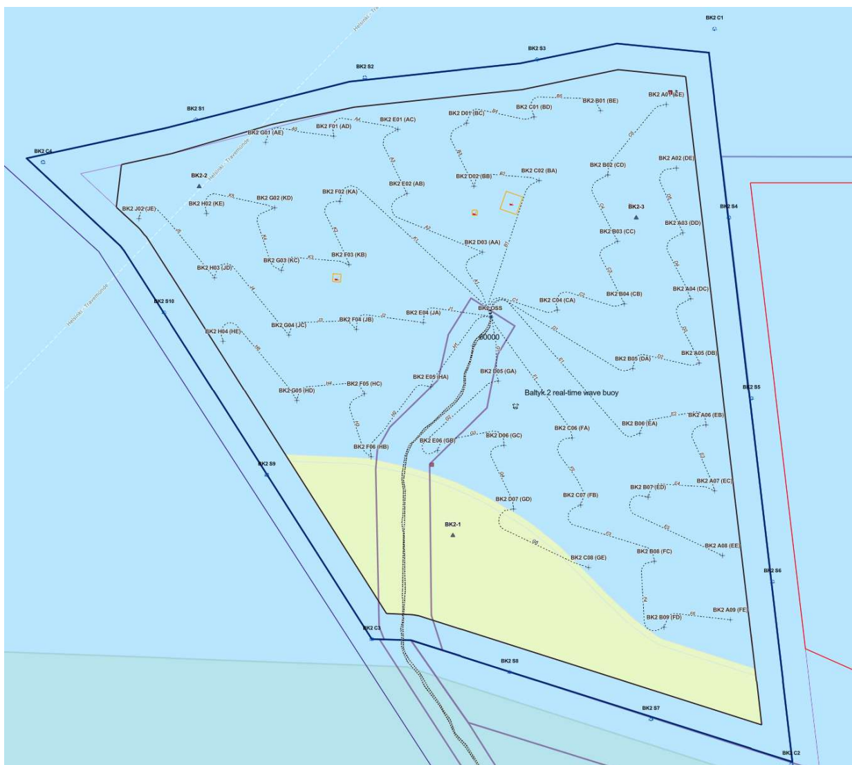
Figure 6 – Bałyk 2 Inter Array Cables Installation Status
