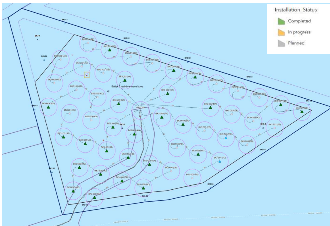
Figure 7 – Bałtyk 3 OWF Installation Overview
