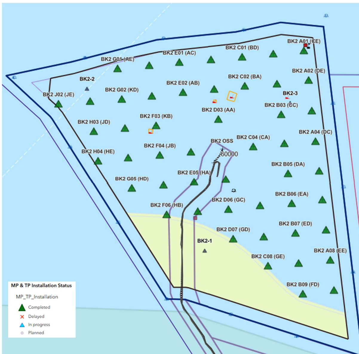
Figure 5 – Bałtyk 2 OWF Installation Overview
