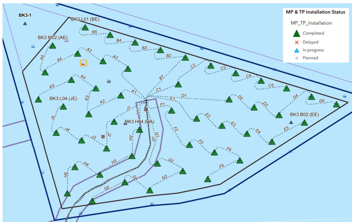
Figure 7 – Bałtyk 3 OWF Installation Overview
