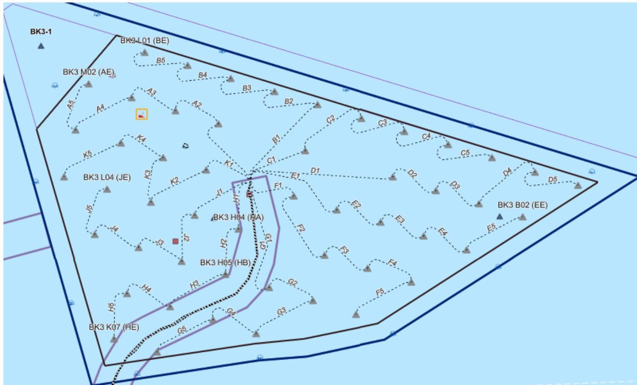
Figure 8 – Bałtyk 3 Inter Array Cables Installation Progress Status
