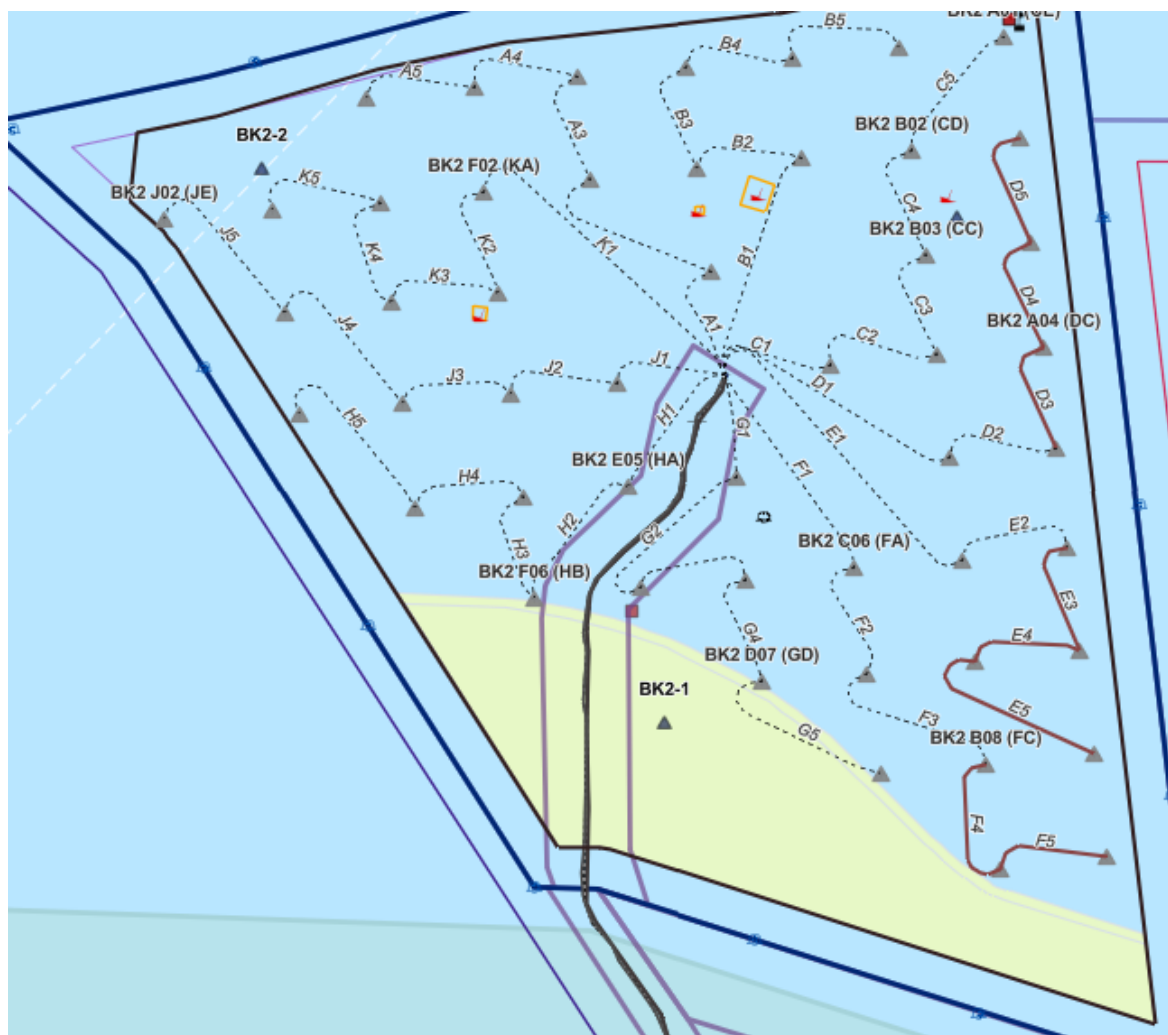
Figure 6 – Bałtyk 2 Inter Array Cables Installation Status
