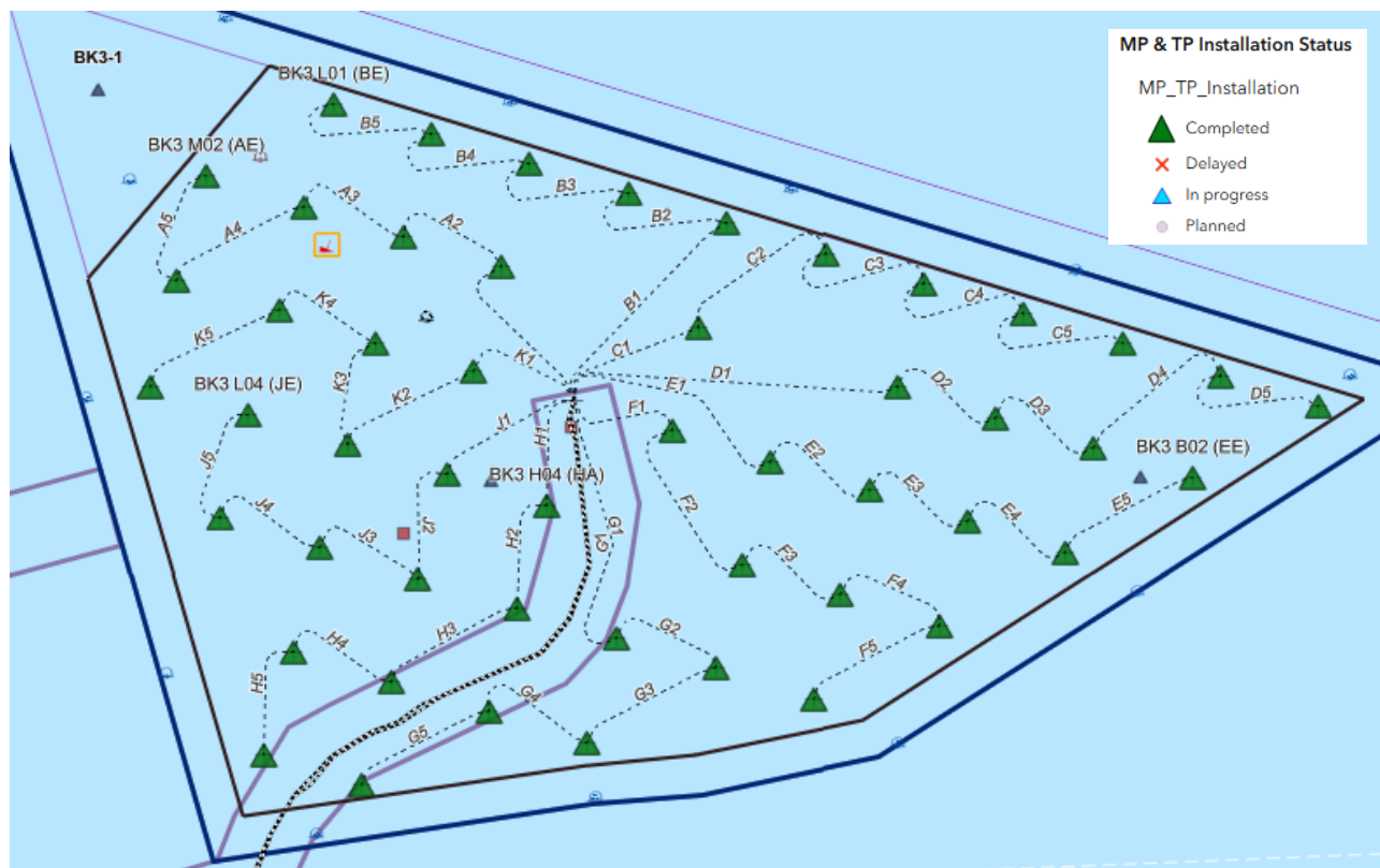
Figure 7 – Bałtyk 3 OWF Installation Overview
