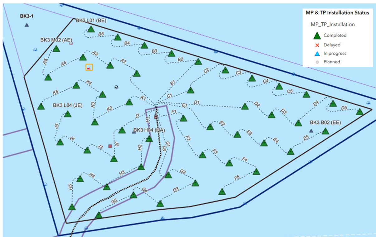
Figure 7 – Bałyk 3 OWF Installation Overview
