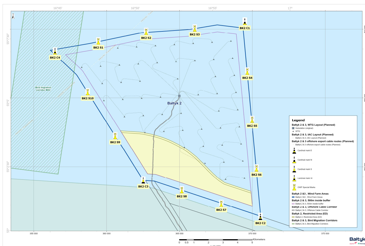
Figure 3 – Layout of demarcation buoys in Bałyk 2 OWF
