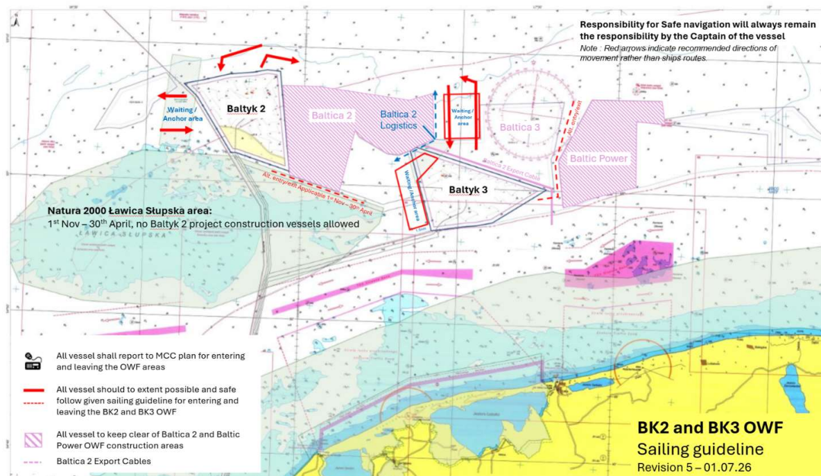
Figure 2 – Layout of the Bałytk 2&3 entry/exit corridors
