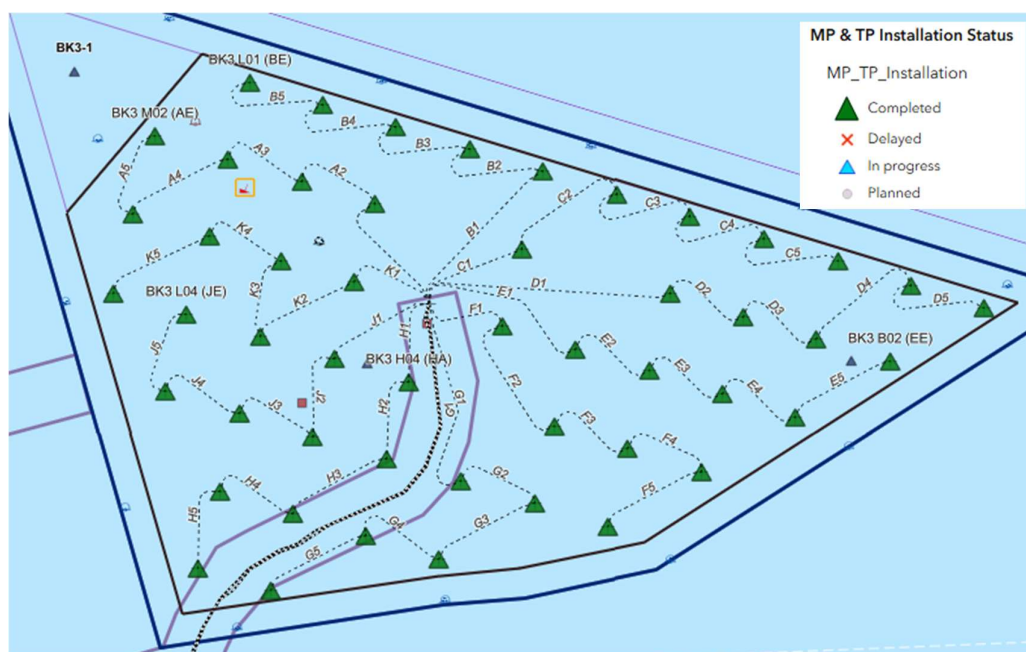
Figure 7 – Bałyk 3 OWF Installation Overview
