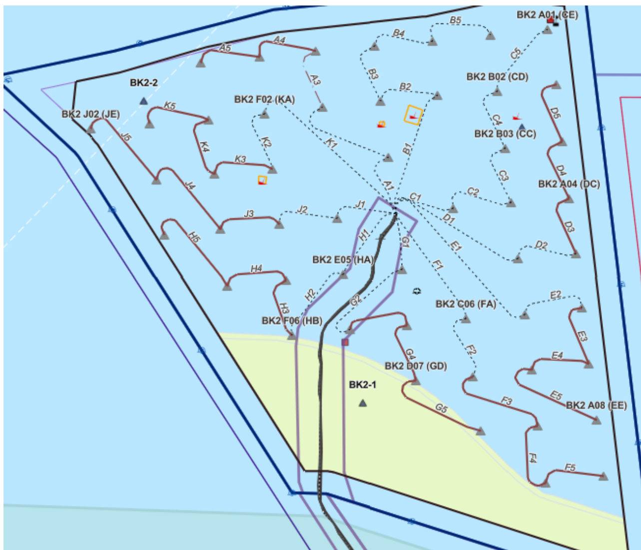
Figure 6 – Bałtyk 2 Inter Array Cables Installation Status
