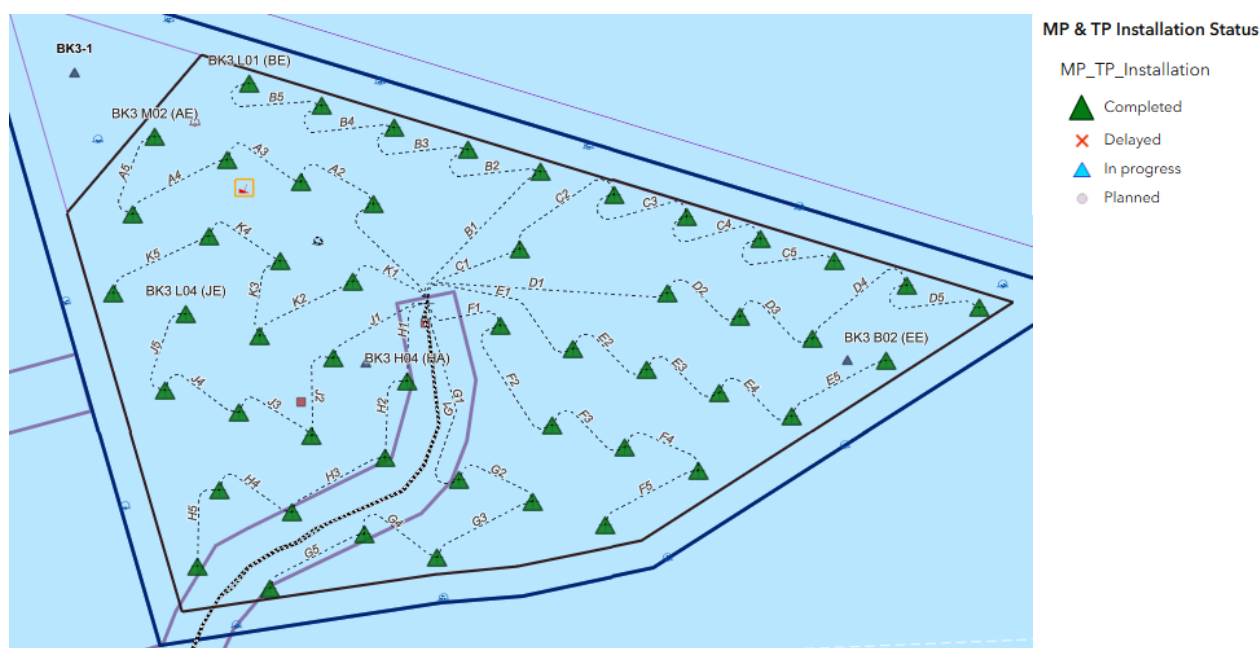
Figure 7 – Bałtyk 3 OWF Installation Overview
