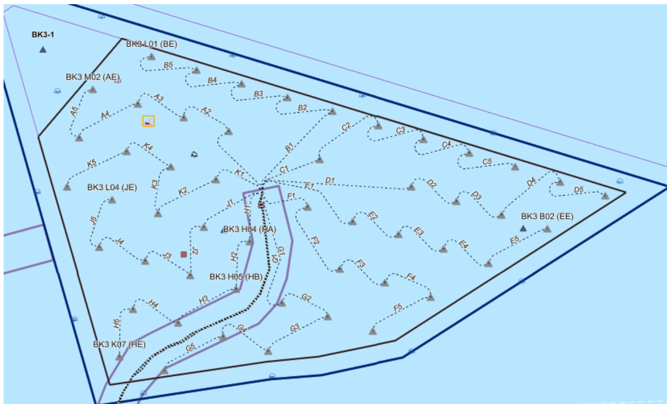
Figure 8 – Bałytk 3 Inter Array Cables Installation Progress Status
